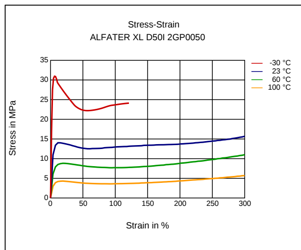
Stress-Strain
